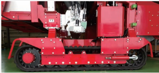
Outstanding stability by long crawler and low center of gravity
